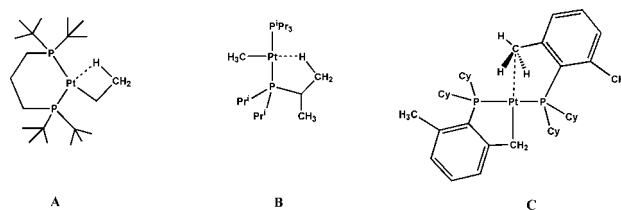
Chart 1. View of Some Cationic T-Shaped Platinum(II) Molecules Stabilized by Agostic Interactions
